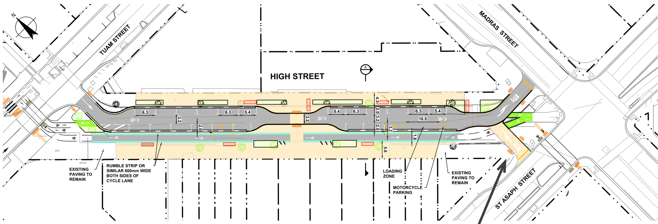
PLAN SCALE 1:500
