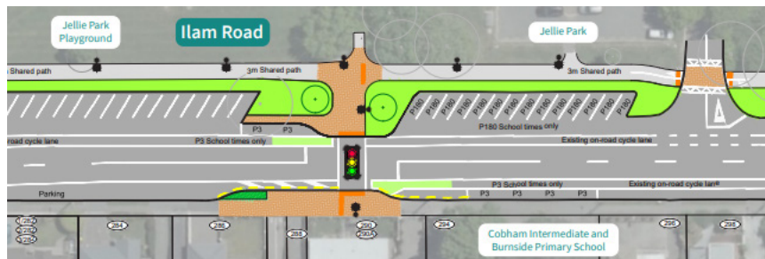
Left: The signalised crossing outside Jellie Park. Below: Visualisation of Ilam Road looking north.
