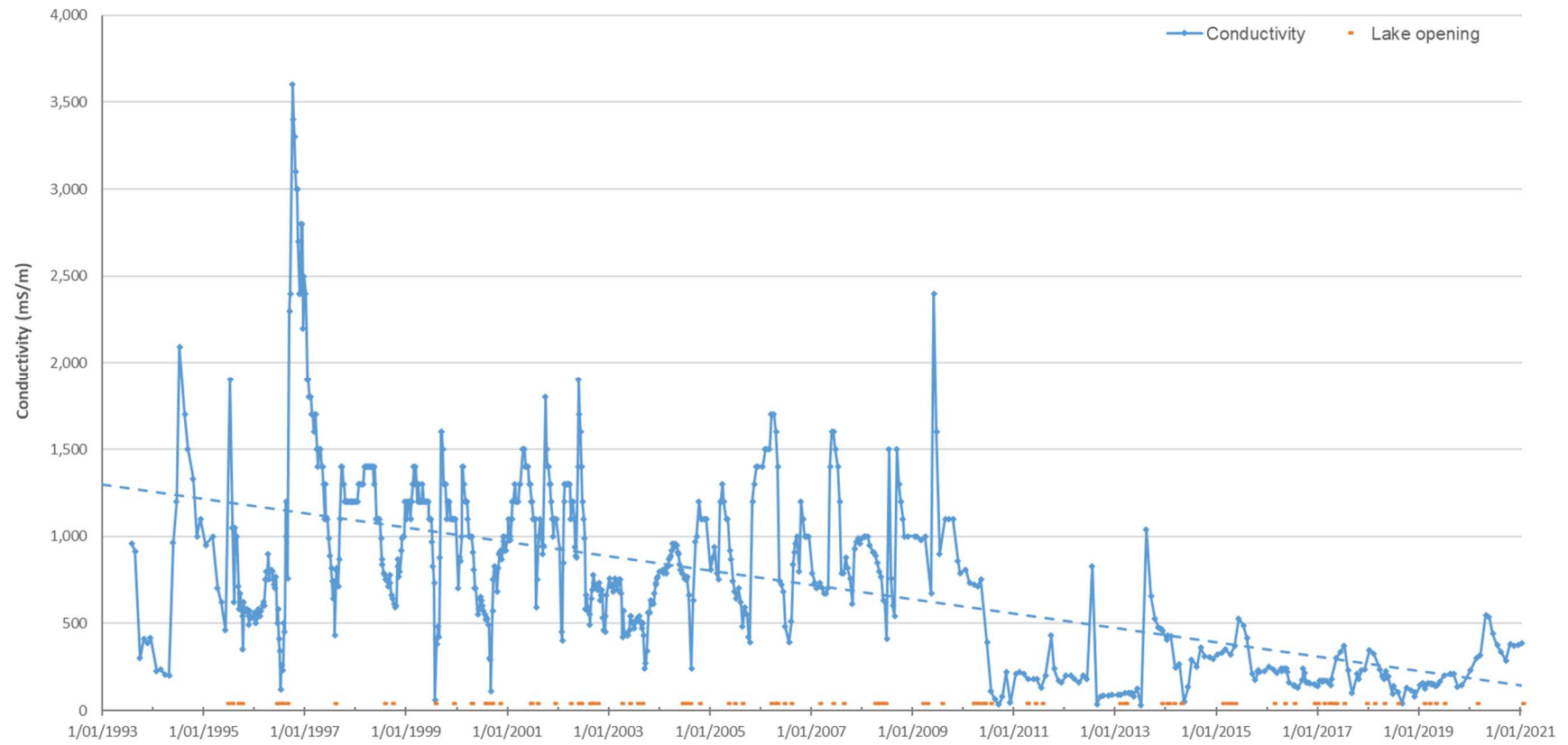
Figure 2. Conductivity of water at Te Wairewa – Lake Forsyth at the ECan Water Level Recorder site July 1993 - December 2021. The dashed line is a linear trendline.
