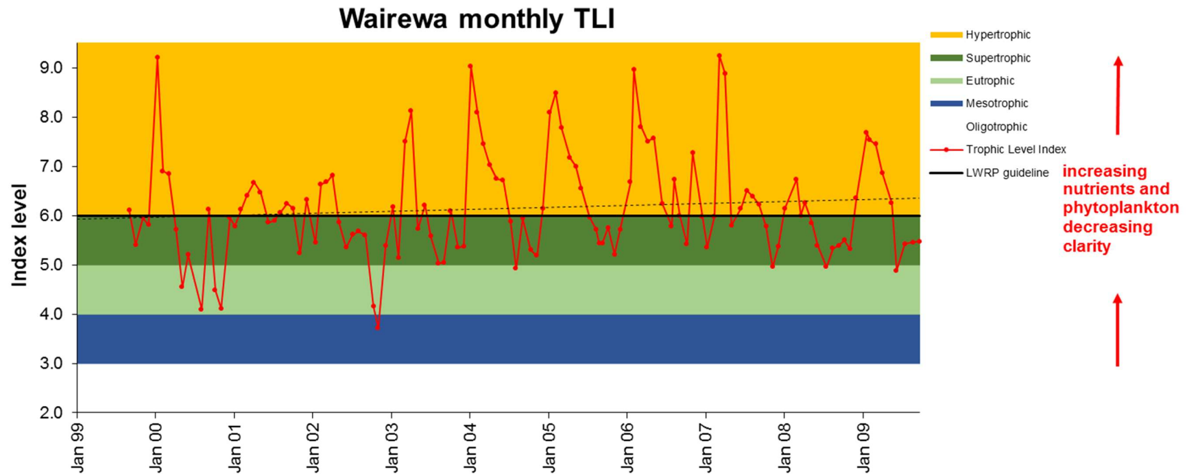
Figure 8b. Trophic Level Index (TLI) at Te Wairewa – Lake Forsyth at the ECan Water Level Recorder site prior to the construction of the canal opening (September 1999 –September 2009). The dashed line is a linear trendline. Solid black line = Land and Water Regional Plan (LWRP) guideline for coastal lakes (6 TLI). Graph modified from ECan versions.
