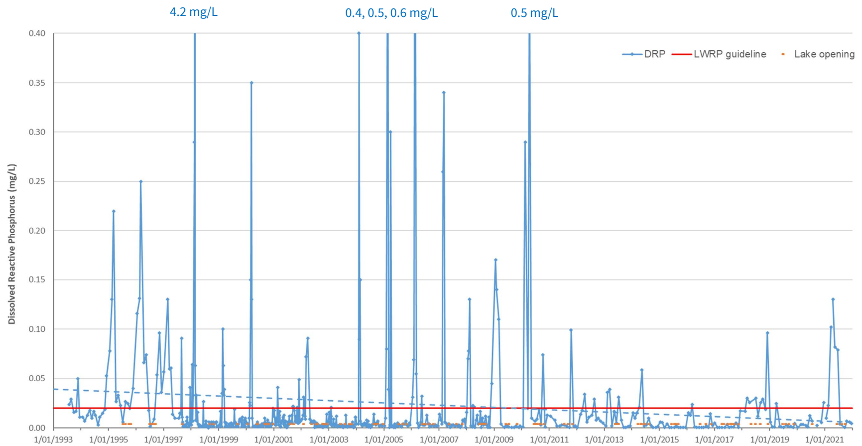
Figure 7. DRP at Te Wairewa – Lake Forsyth at the ECan Water Level Recorder site July 1993 – December 2021. The dashed line is a linear trendline. Five data points are substantially higher than the other data points and are therefore off the scale of the graph – the numbers above the graph detail their concentrations.
