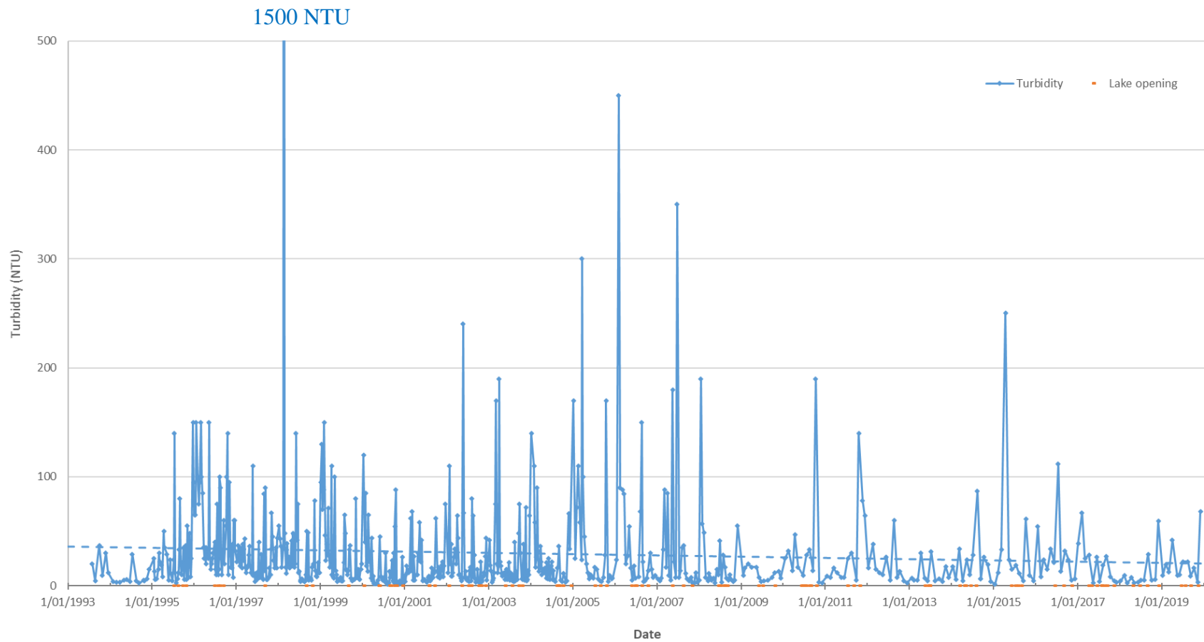
Figure 5. Turbidity of water at Wairewa/Lake Forsyth at the water level recording site for the entire dataset (July 1993 - December 2019). The dashed line is a linear trendline. One data point is substantially higher than the other data points and is therefore off the scale of the graph – number above the graph detail the concentration.
