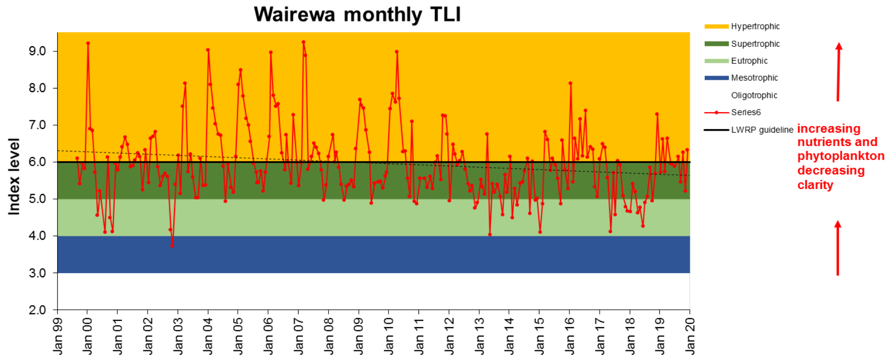
Figure 8a. Trophic Level Index (TLI) at Wairewa/Lake Forsyth at the ECan Water Level Recorder site for the entire dataset (September 1999 – December 2019). The dashed line is a linear trendline. Solid black line = Land and Water Regional Plan (LWRP) guideline for coastal lakes (6). Graph modified from ECan versions.
