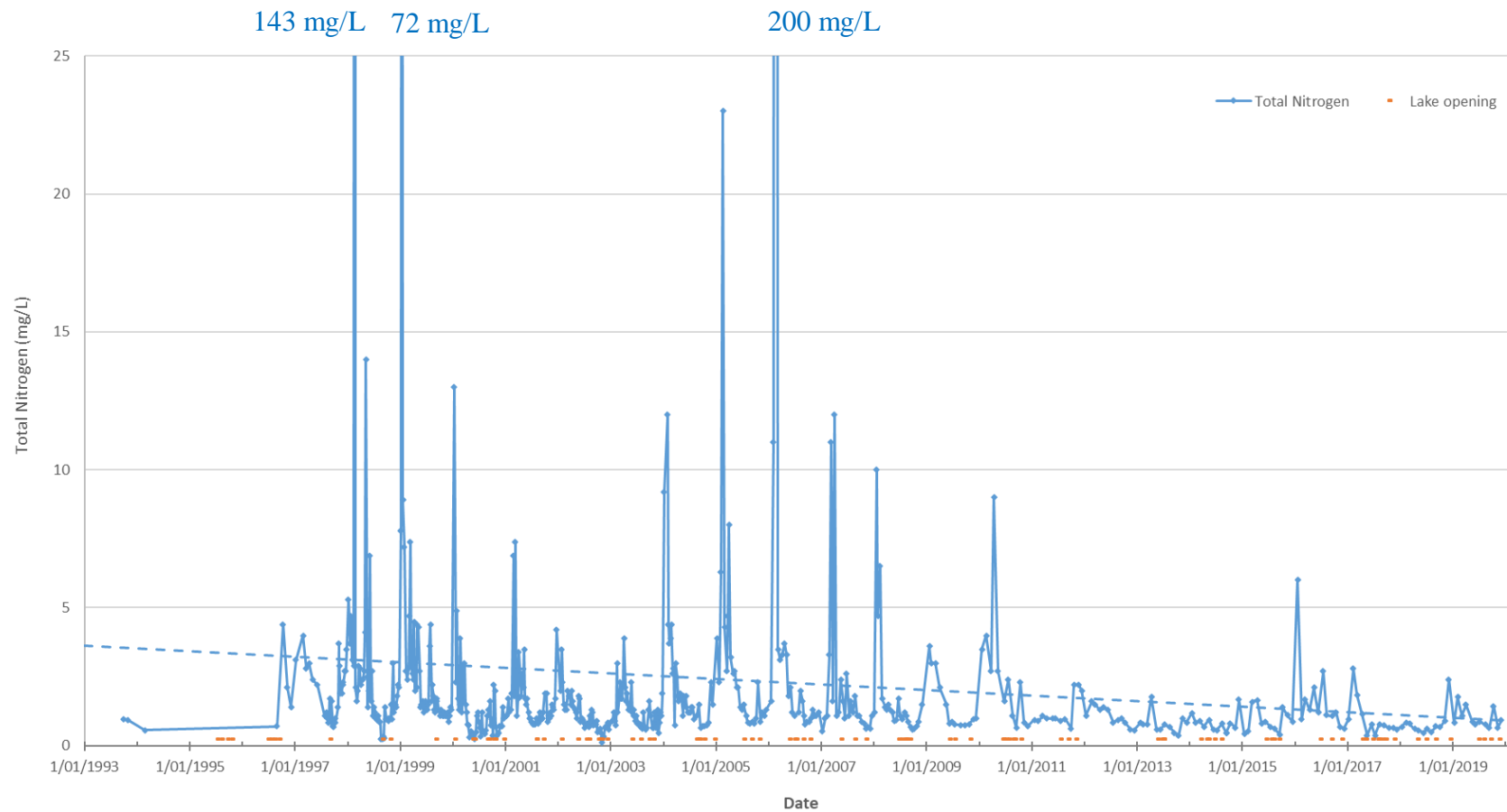
Figure 6. Total Nitrogen at Wairewa/Lake Forsyth at the ECan Water Level Recorder site for the entire dataset (July 1993 – December 2019). The dashed line is a linear trendline. Three data points are substantially higher than the other data points and are therefore off the scale of the graph – the numbers above the graph detail their concentrations.
