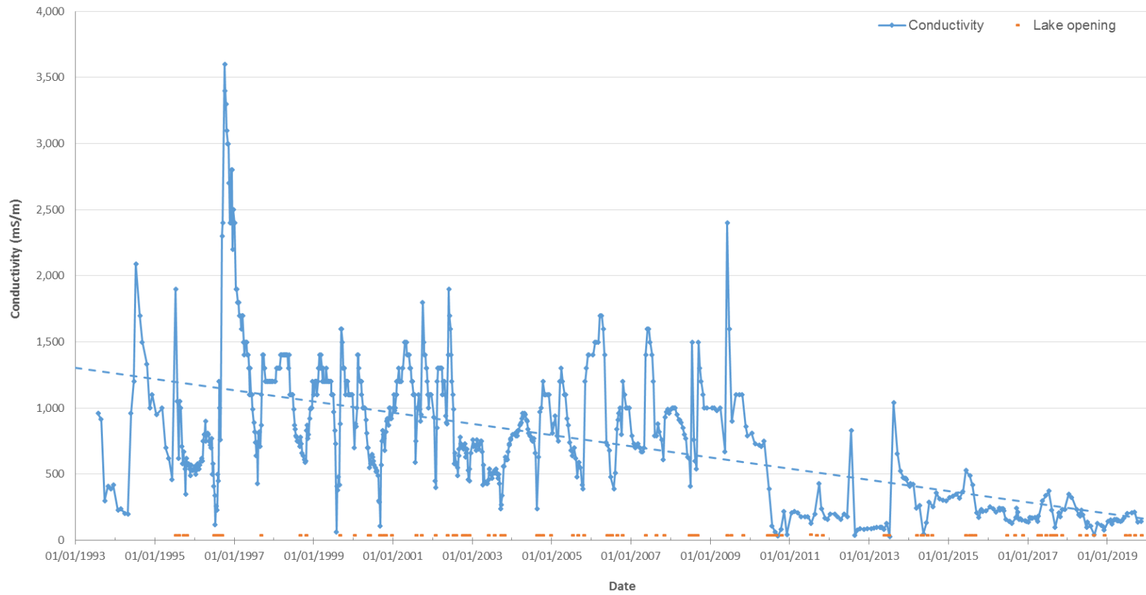
Figure 2. Conductivity of water at Wairewa/Lake Forsyth at the ECan Water Level Recorder site for the entire dataset (July 1993 - December 2019). The dashed line is a linear trendline.
