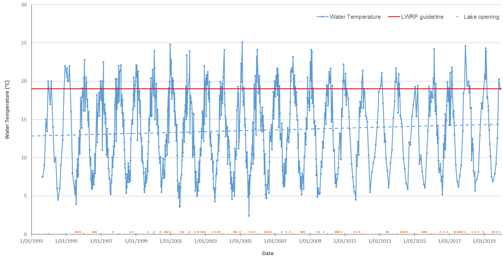
Figure 4. Water Temperature at Wairewa/Lake Forsyth at the ECan Water Level Recorder site for the entire dataset (August 1993 - December 2019). The dashed line is a linear trendline. Red line = Land and Water Regional Plan (LWRP) guideline for coastal lakes (19°C).
