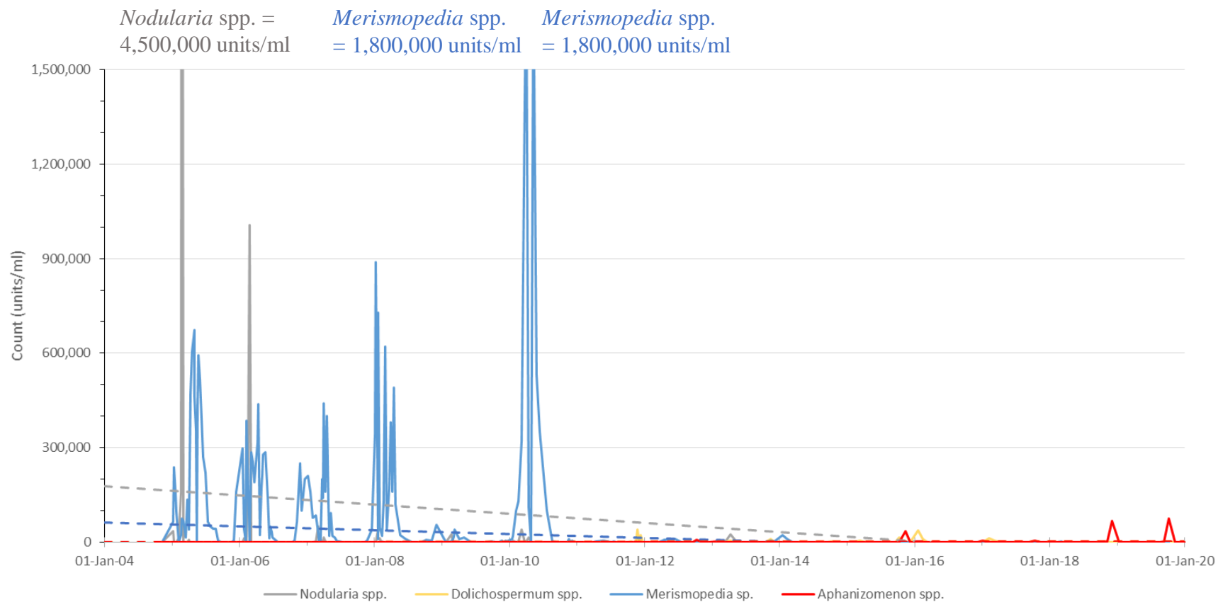
Figure 10. Counts at Wairewa/Lake Forsyth at the ECan Water Level Recorder site for the potentially toxic cyanobacteria Nodularia spp., Dolichospermum spp., Merismopedia spp. and Aphanizomenon spp. from September 2004 to December 2019. The dashed lines are linear trendlines. Three data points are significantly higher than the other data points and are therefore off the scale of the graph – the numbers above the graph detail their concentrations.
