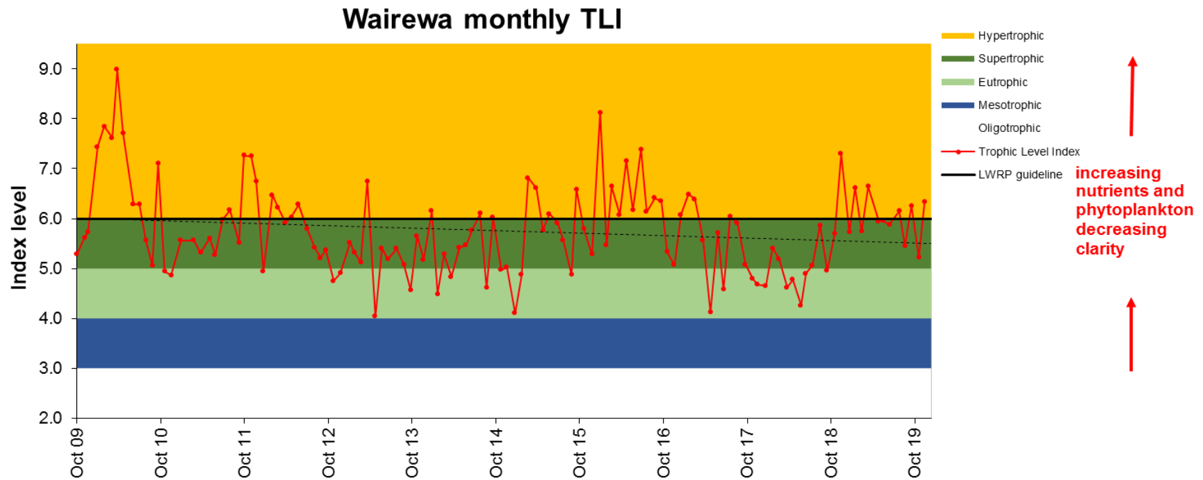
Figure 8c. Trophic Level Index (TLI) at Wairewa/Lake Forsyth at the ECan Water Level Recorder site after the construction of the canal opening (October 2009– December 2019). The dashed line is a linear trendline. Solid black line = Land and Water Regional Plan (LWRP) guideline for coastal lakes (6). Graph modified from ECan versions.
