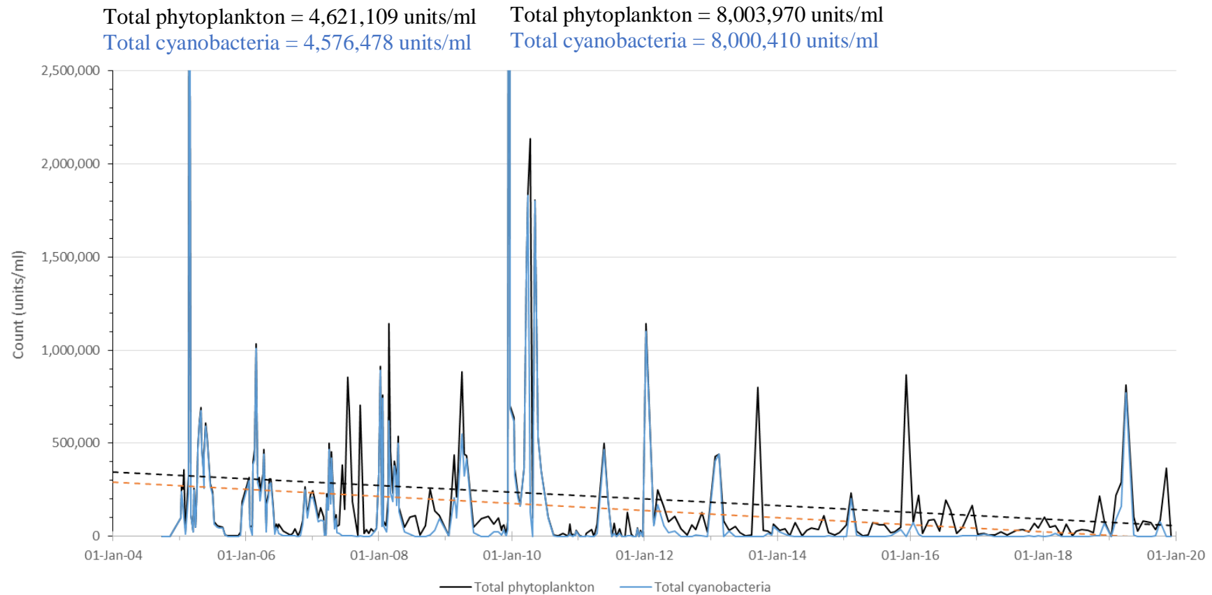
Figure 9. Total phytoplankton and cyanobacteria counts at Wairewa/Lake Forsyth at the ECan Water Level Recorder site from September 2004 to December 2019. The dashed lines are linear trendlines. Two data points are significantly higher than the other data points and are therefore off the scale of the graph – the numbers above the graph detail their concentrations.
