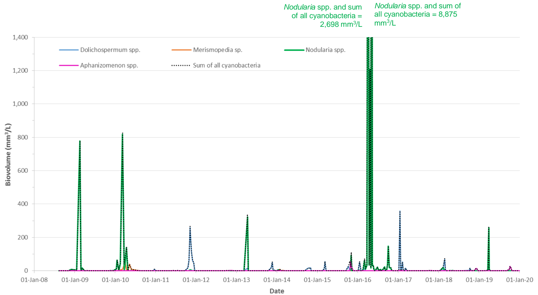
Figure 11. Biovolumes of potentially toxic cyanobacteria Nodularia spp., Dolichospermum spp., Merismopedia spp., Aphanizomenon spp. and the sum of all cyanobacteria at Wairewa/Lake Forsyth at the ECan Water Level Recorder site from August 2008 – December 2019. Two data points are significantly higher than the other data points and are therefore off the scale of the graph – the numbers above the graph detail their concentrations.
