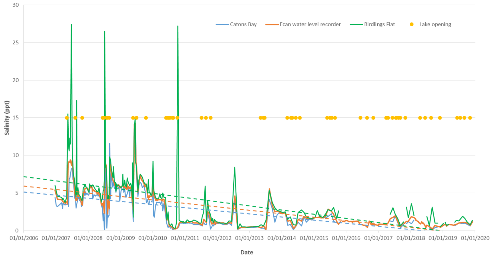
Figure 3. Salinity of water at Wairewa/Lake Forsyth at three sites (ECan Water Level Recorder, Catons Bay and Birdlings Flat) from the entire dataset (December 2006 - December 2019). The dashed lines are linear trendlines.
