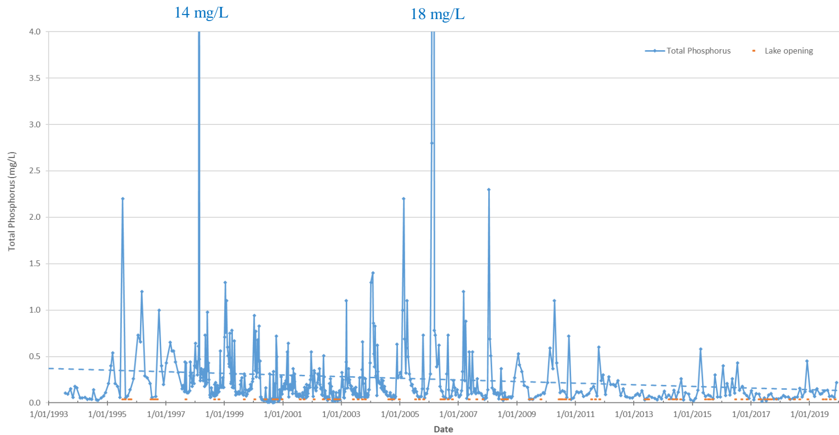
Figure 7. Total phosphorus at Wairewa/Lake Forsyth at the ECan Water Level Recorder site for the entire dataset (July 1993 – December 2019). The dashed line is a linear trendline. Two data points are substantially higher than the other data points and are therefore off the scale of the graph – the numbers above the graph detail their concentrations.
