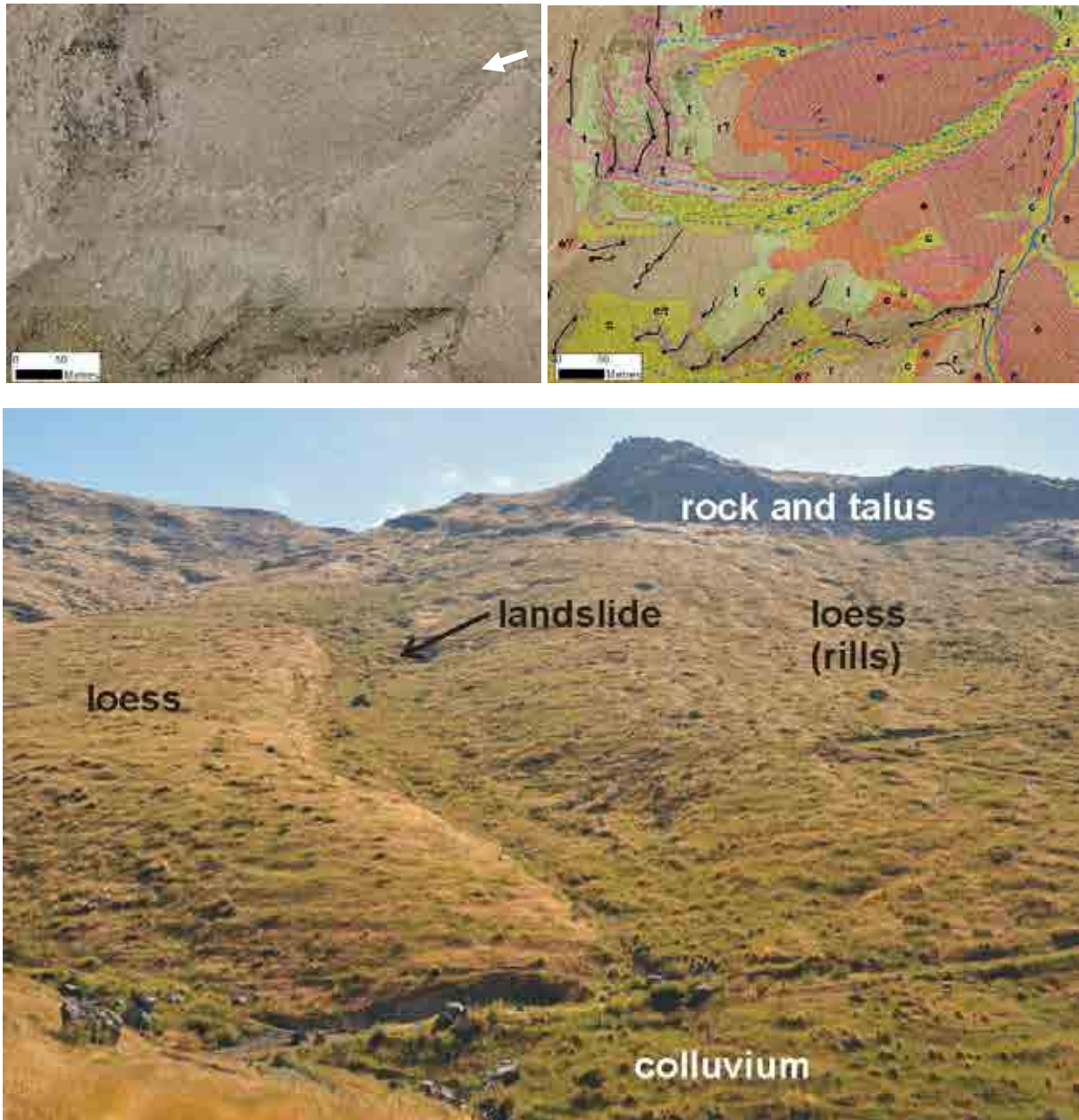
Figure 10 A landslide of shallow earthflow type in the Horotane Valley fills the small gully in the centre left. The rounded ridges on either side consist of loess. Note also the large boulders on the valley floor, many of which have fallen from Castle Rock (to the left, out of the picture) (Grid Reference 1575000/5174300).
