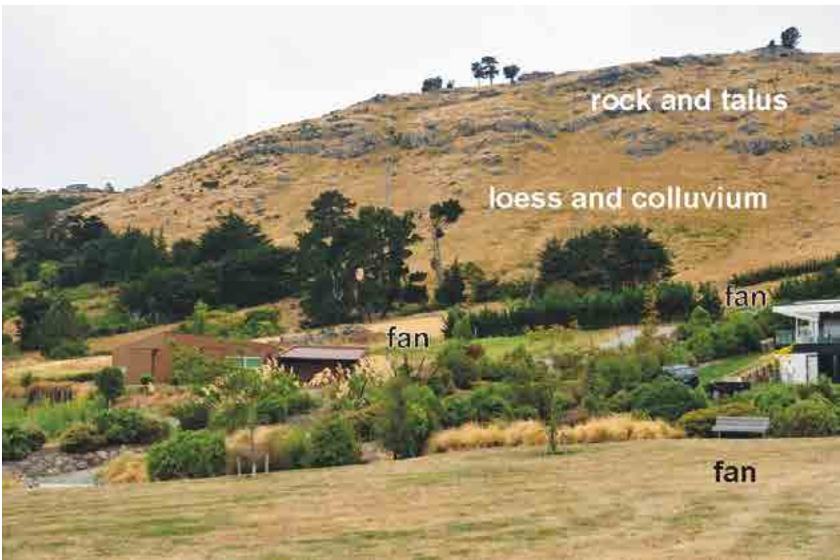
Figure 9 Colluvial fans forming gently dipping surfaces below steep rock cliffs in the Heathcote Valley (Grid Reference 1577100/5175000).
