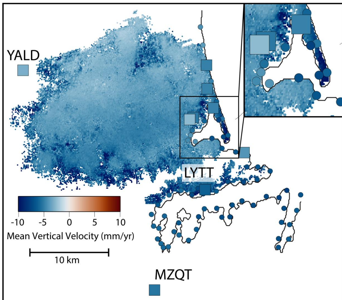
Figure 3.1 Best-fitting displacement rate over Christchurch between April 2016 and August 2021 based on PhD analysis of Jesse Kears. Mean rates have been adjusted to match the average vertical deformation at GNSS sites across Christchurch (coloured squares). Labelled GNSS sites are from the national network, whose timeseries are shown in Figure 3.3. The subplot in the top right shows a zoom-in of the New Brighton / Southshore area.
