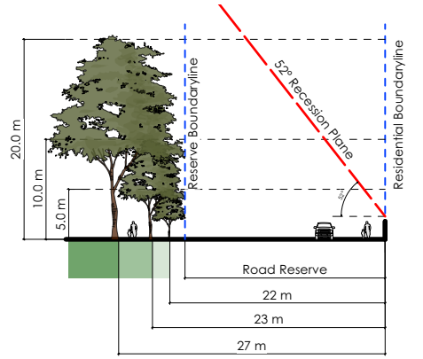
Cross Section E-E
