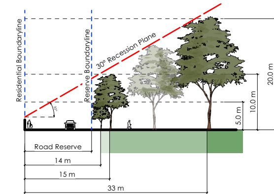
Cross Section E-E
