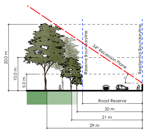
Cross Section C-C (18m Road)
