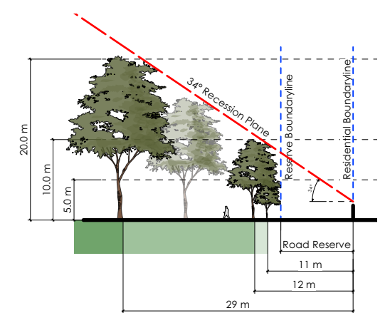
Cross Section D-D (9m Road)
