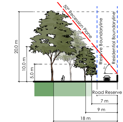
Cross Section F-F
