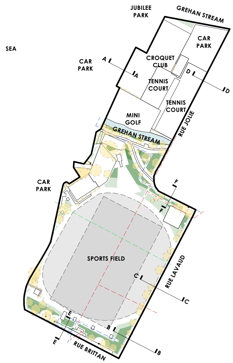
Location Plan @ 1:2000
