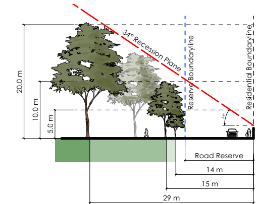
Cross Section B-B (12m Road)
