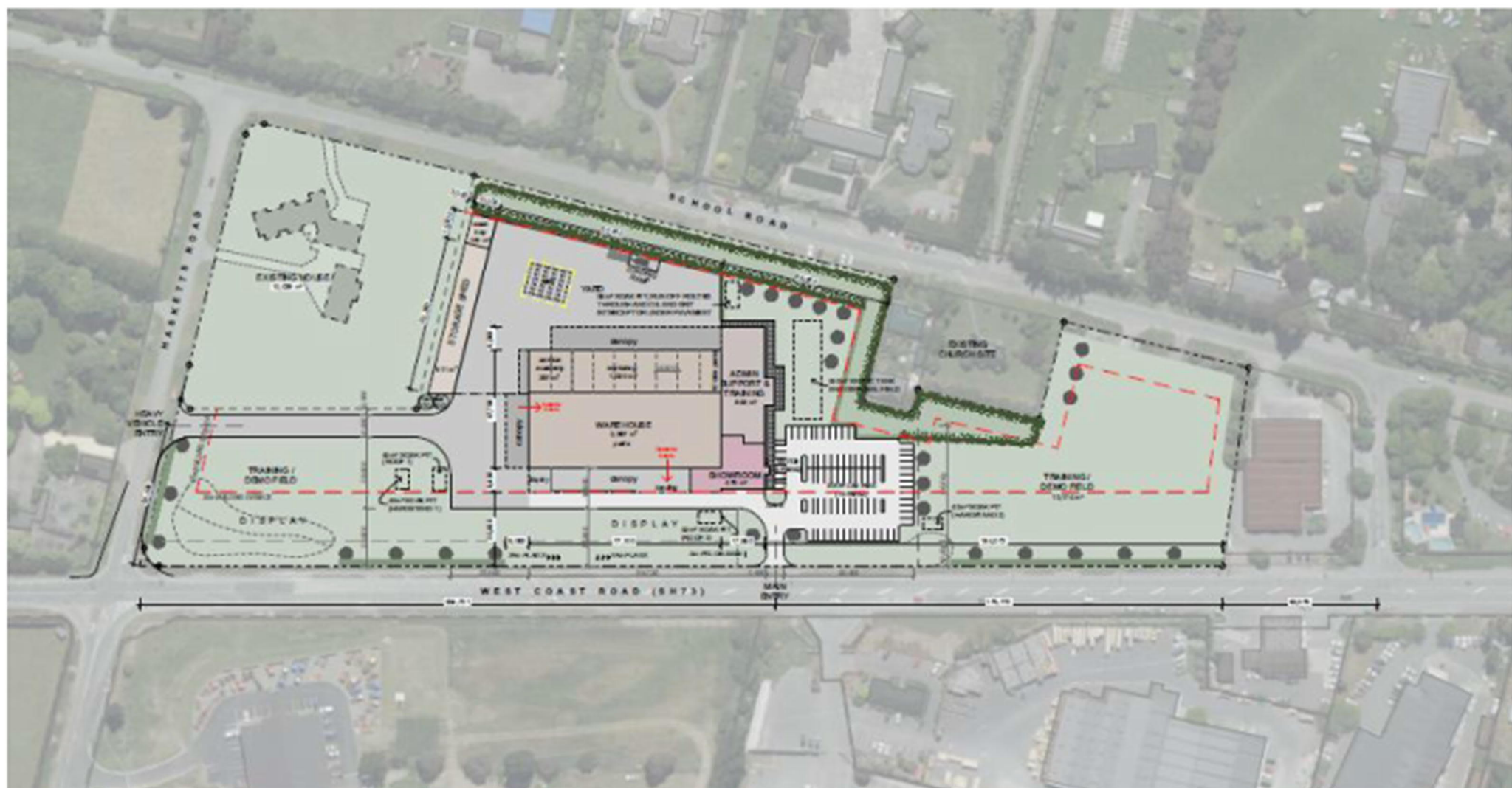
Figure 5: Proposed Site Layout.
