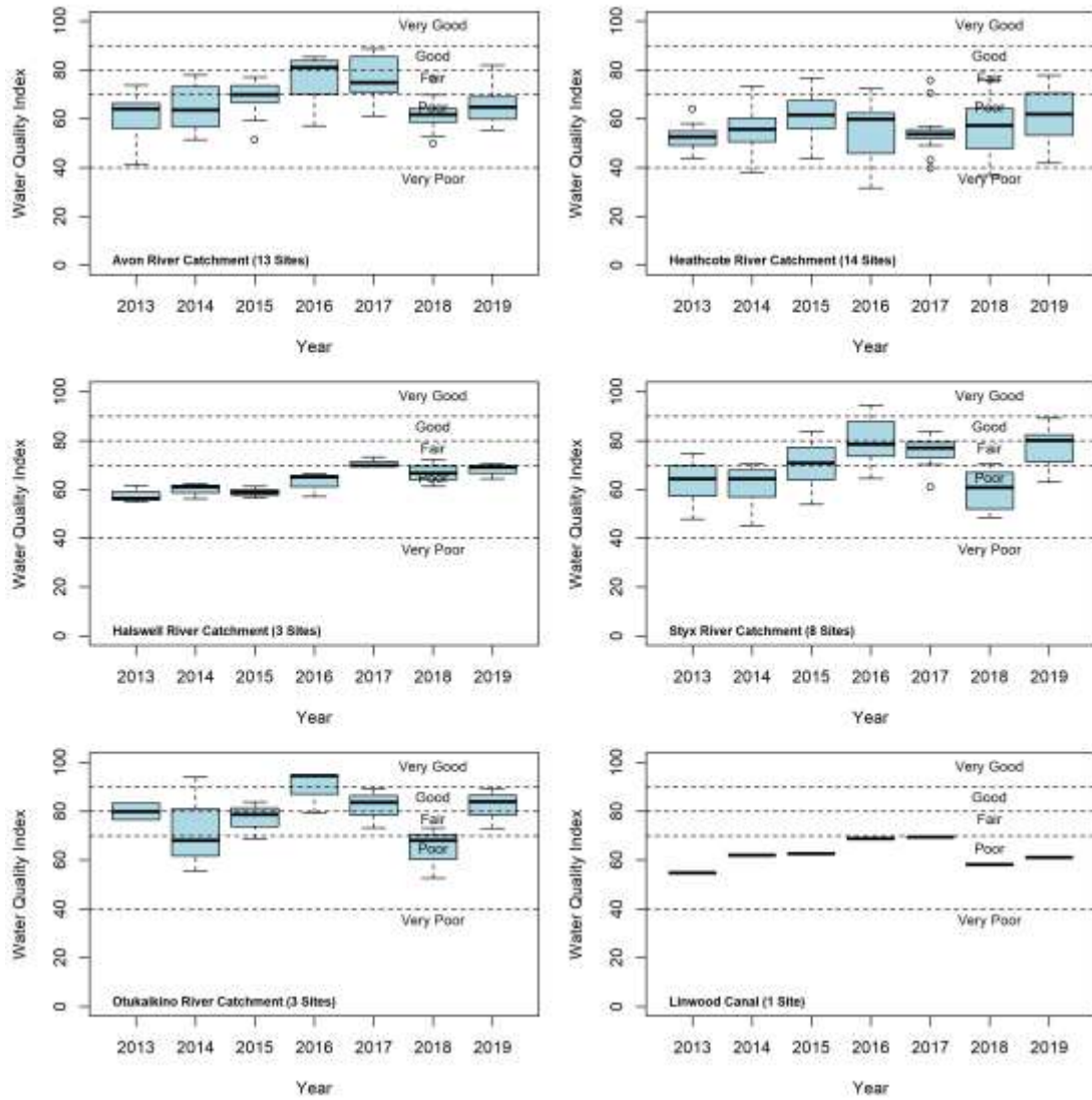
Figure 8: Water Quality Index for each catchment for the 2013 to 2019 monitoring years
