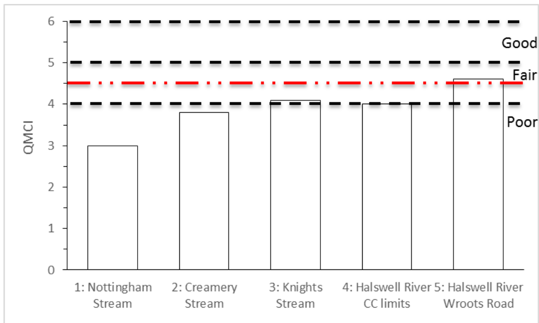
Figure 9: Macroinvertebrate Community Index (MCI) scores (top) and QMCI scores (bottom)
