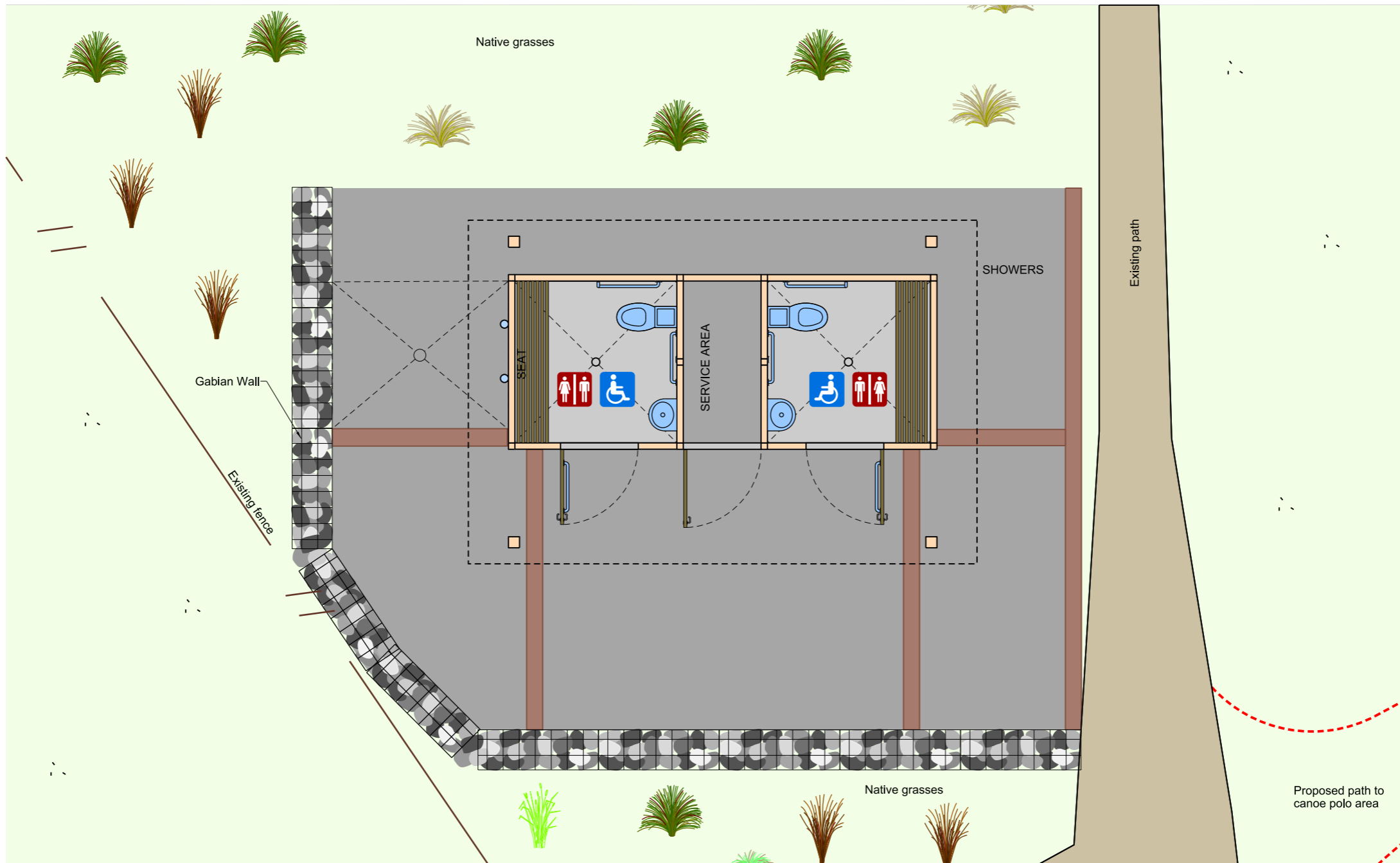
PLAN NTS
