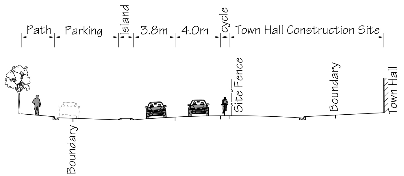
A Typical Cross Section - Current Layout Not to Scale
