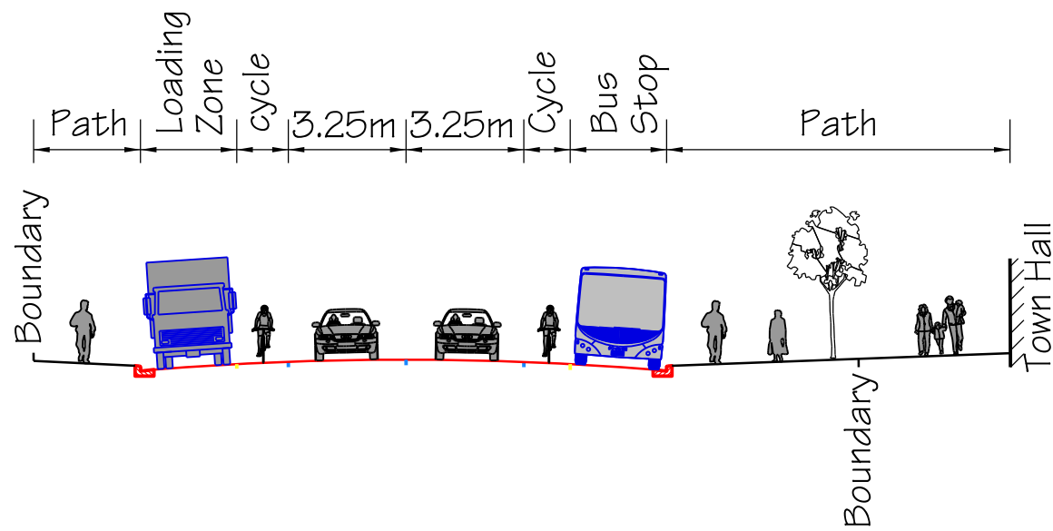
A Cross Section at Bus Stops - Phase 1 Not to Scale
