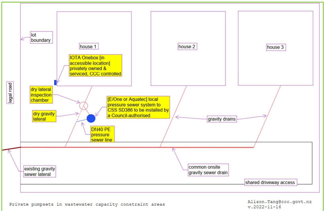
Figure 3 – LPSS location in a capacity constraint area
