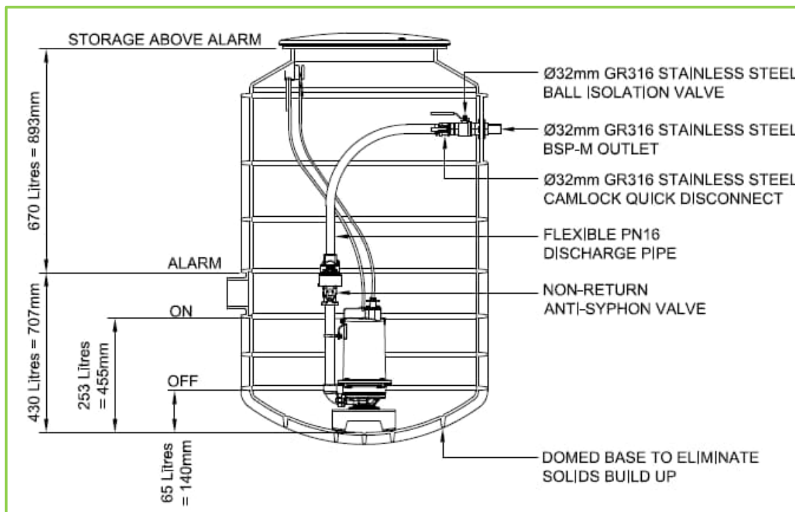
Figure 2 – Pump Chamber Operating Range
