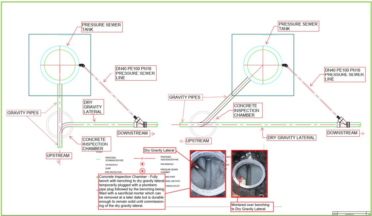
Figure 8 – Dry gravity lateral connection details
